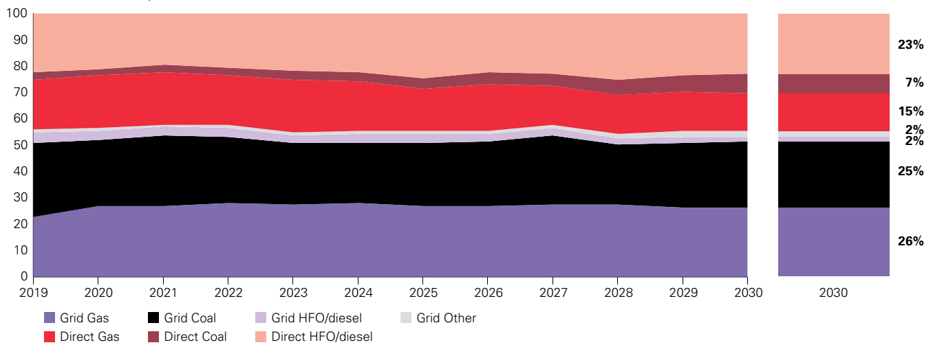
Chart 19: Breakdown of power sources and emissions to 2030
