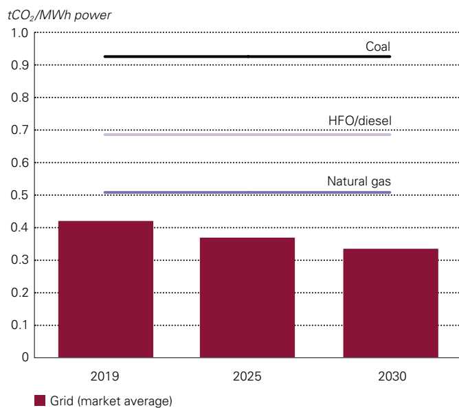
Chart 5: Grid emissions intensity by power supply type
